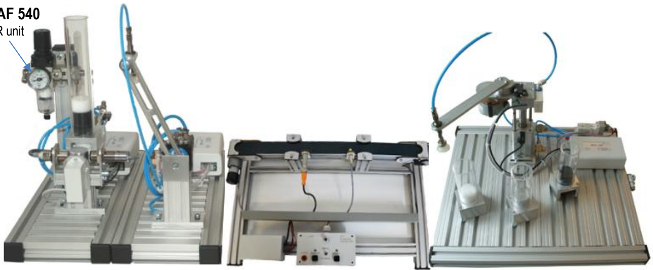
MAF 500 Gravity feeder with part detection
