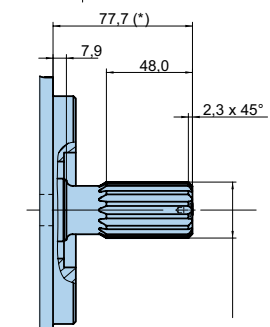
SHAFT CODE 4
