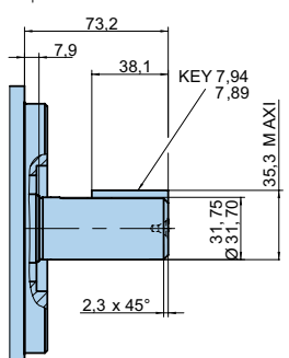
SHAFT CODE 2
