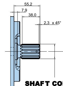
SHAFT CODE 3
