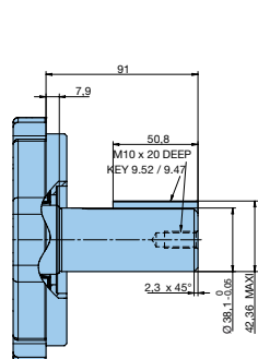
SHAFT CODE 2 (KEYED SAE CC)
