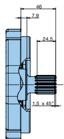
SHAFT CODE 4 SAE BB INVOLUTE SPLINE DATA CLASS 1 - FLAT ROOT SIDE FIT J4989 - PITCH 16/32 15 TEETH - 30° PRESSURE ANGLE
